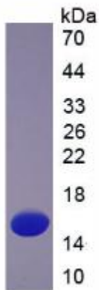
SDS-PAGE Image
