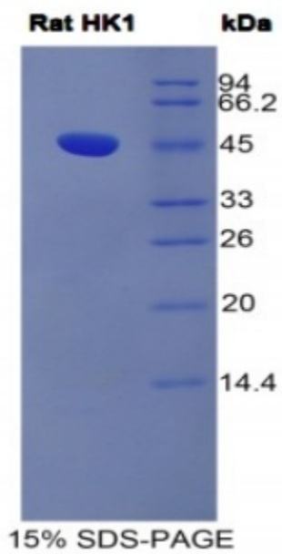
SDS-PAGE Image
