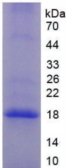
SDS-PAGE Image
