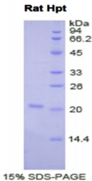
SDS-PAGE Image
