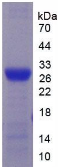
SDS-PAGE Image
