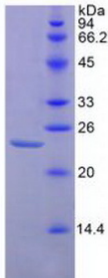
SDS-PAGE Image
