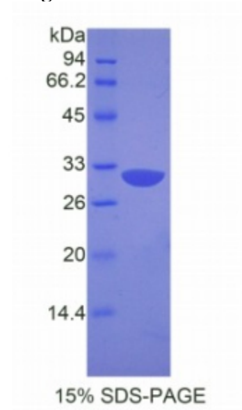
SDS-PAGE Image
