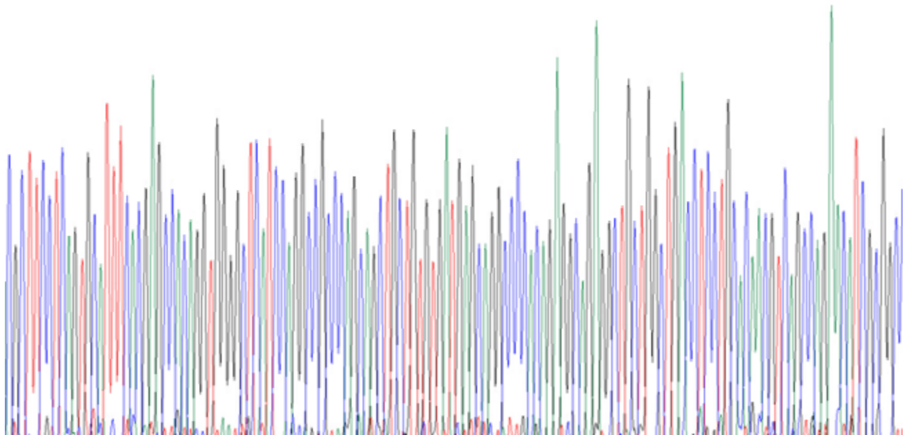
SDS-PAGE Image
