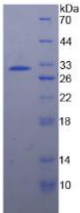
SDS-PAGE Image
