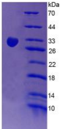
Figure. SDS-PAGE
