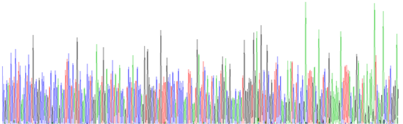
SDS-PAGE Image
