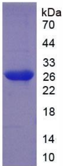
Figure. SDS-PAGE
