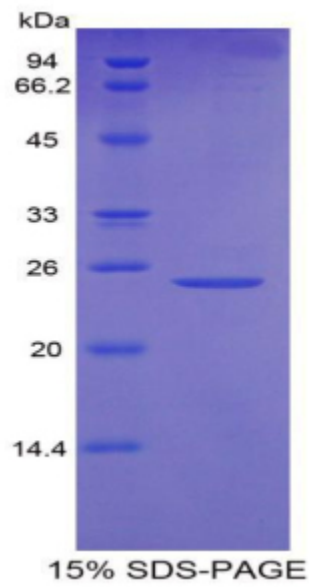
SDS-PAGE Image
