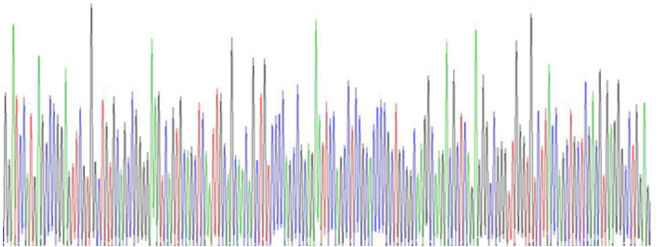
SDS-PAGE Image
