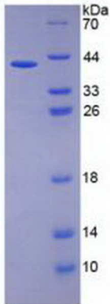
Figure. SDS-PAGE
