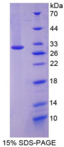
SDS-PAGE Image
