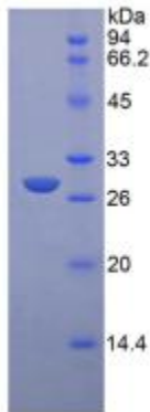
SDS-PAGE Image
