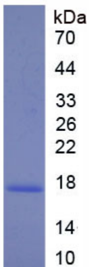
Figure. SDS-PAGE
