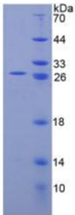
SDS-PAGE Image
