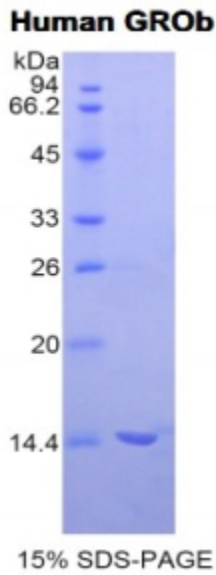
SDS-PAGE Image
