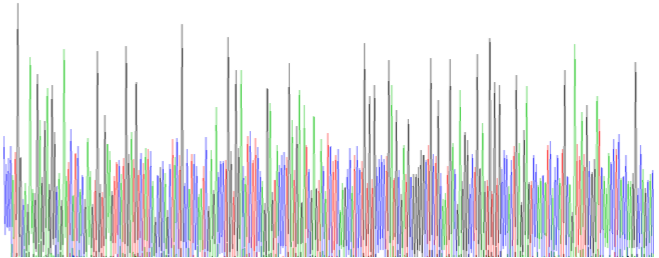
Figure. SDS-PAGE
