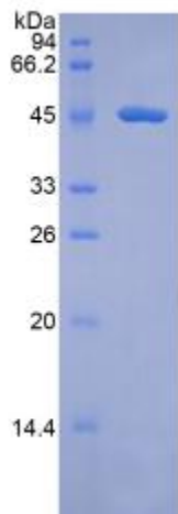
SDS-PAGE Image
