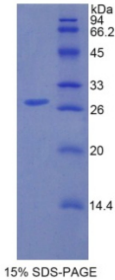
SDS-PAGE Image
