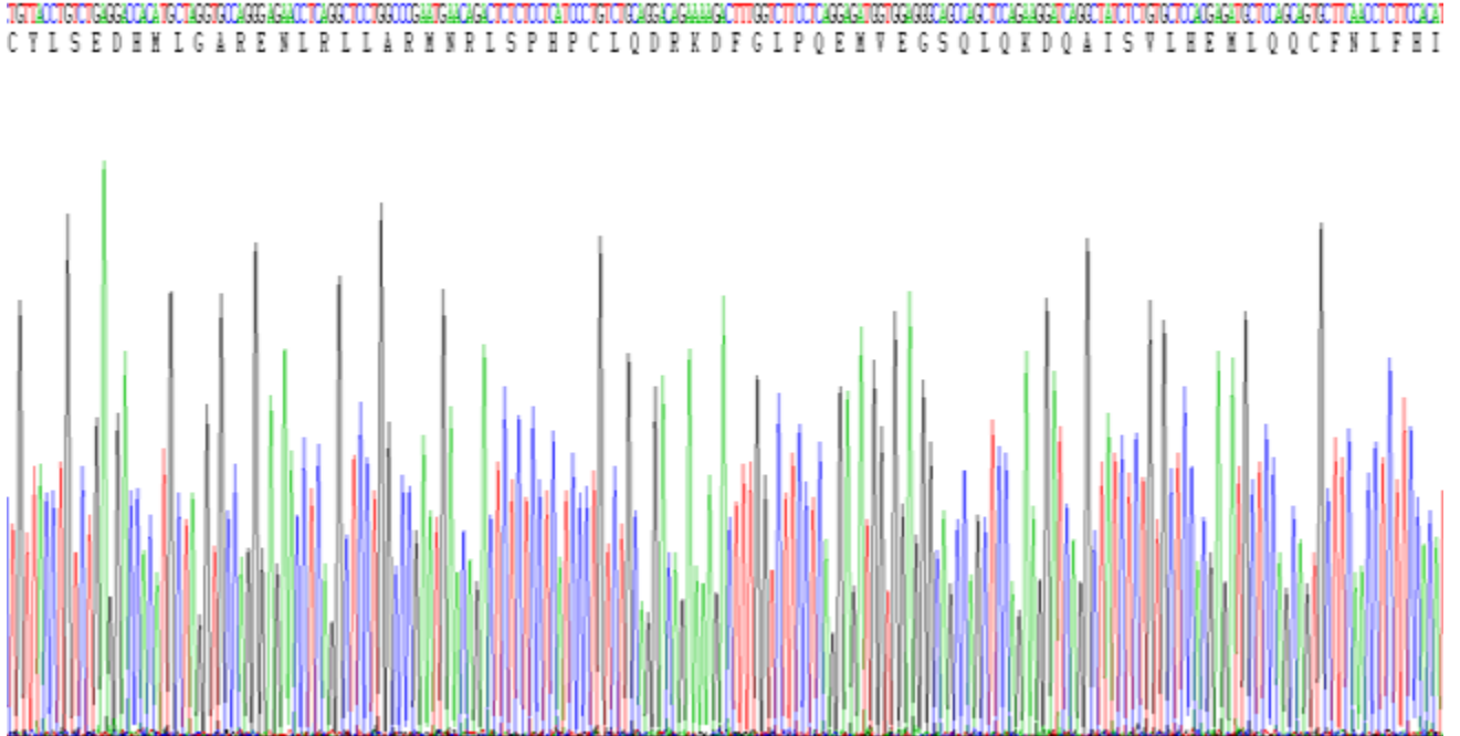
Figure. SDS-PAGE
