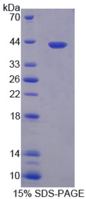
SDS-PAGE Image
