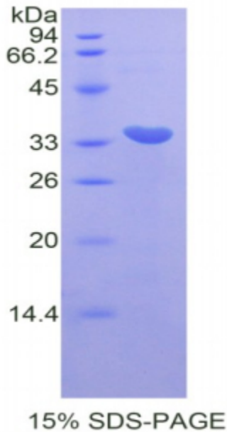
SDS-PAGE Image
