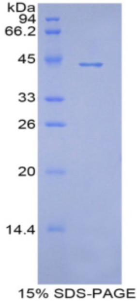
SDS-PAGE Image
