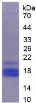
SDS-PAGE Image
