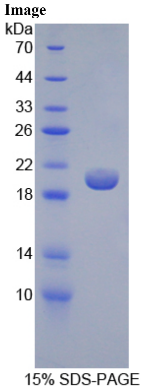
SDS-PAGE Image
