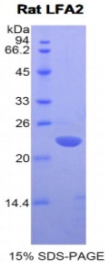
SDS-PAGE Image
