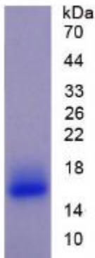
SDS-PAGE Image
