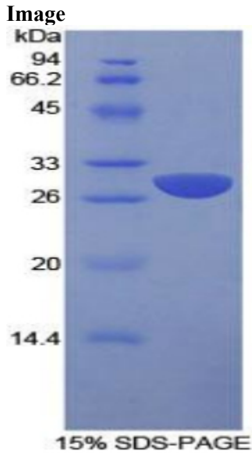
SDS-PAGE Image
