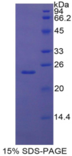
SDS-PAGE Image
