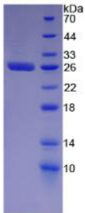
SDS-PAGE Image
