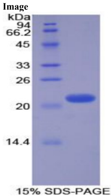
SDS-PAGE Image
