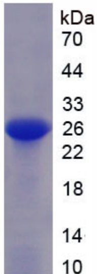
Figure. SDS-PAGE
