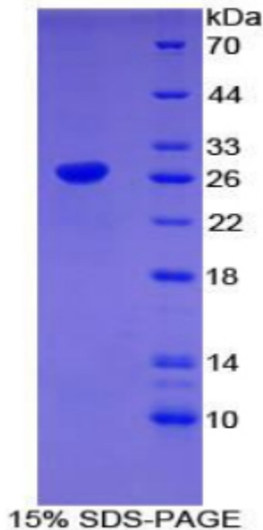
Figure. SDS-PAGE
