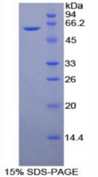
SDS-PAGE Image
