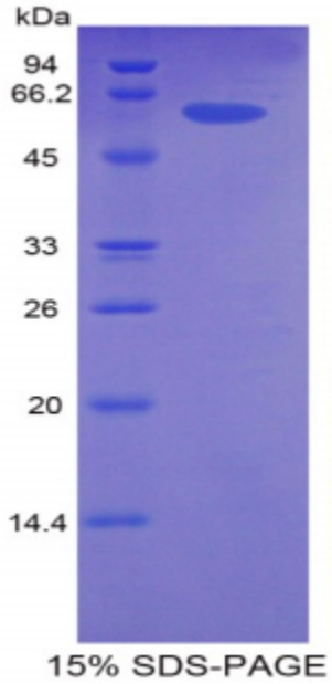
SDS-PAGE Image
