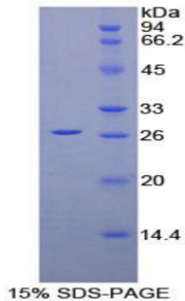
Figure. SDS-PAGE
