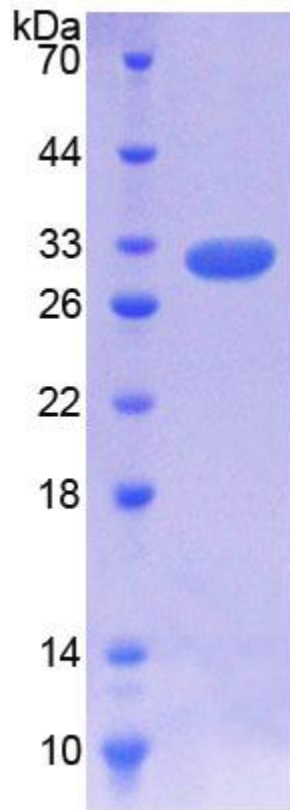
SDS-PAGE Image
