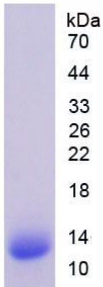
SDS-PAGE Image
