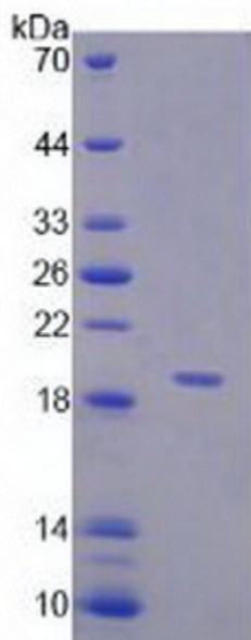
Figure. SDS-PAGE
