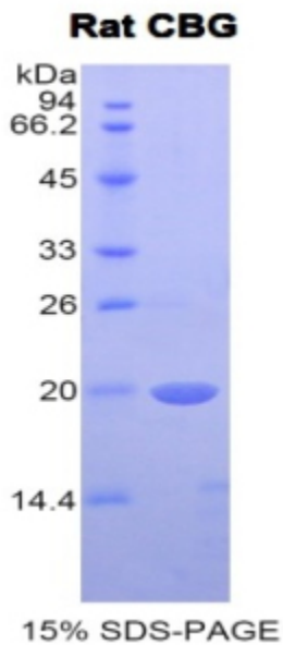
SDS-PAGE Image
