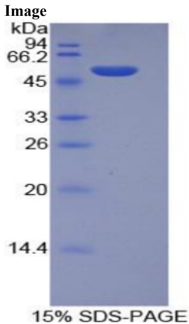
Figure. SDS-PAGE
