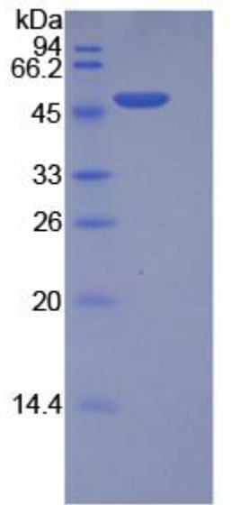
SDS-PAGE Image
