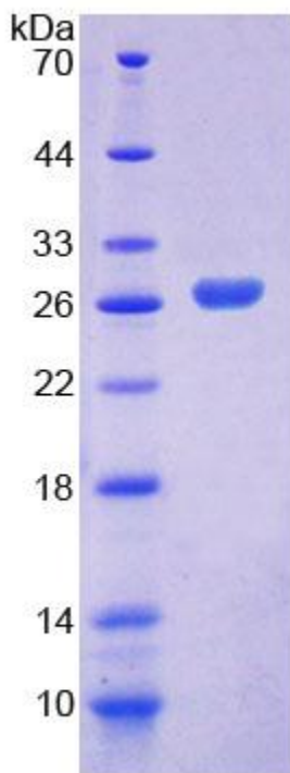
Figure. SDS-PAGE
