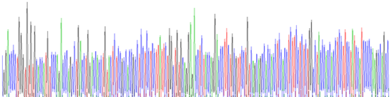
Figure. SDS-PAGE
