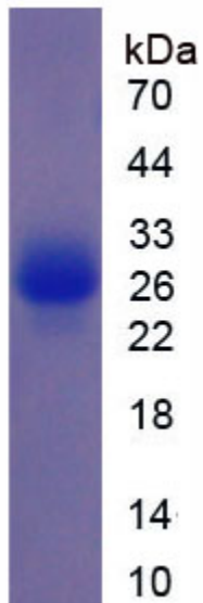
Figure. SDS-PAGE
