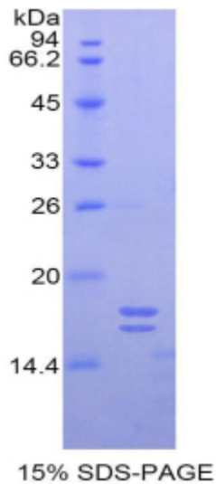
Figure. SDS-PAGE
